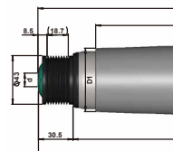
Internal Thread
