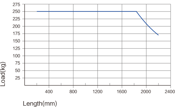
■ Steel tube Φ80x3.0, shaft Φ20, internal thread Steel tube Φ76x3.0, shaft Φ20, internal thread
