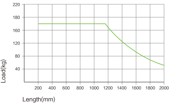
■ Steel tube Φ60x2.0, shaft Φ12/15, internal thread
